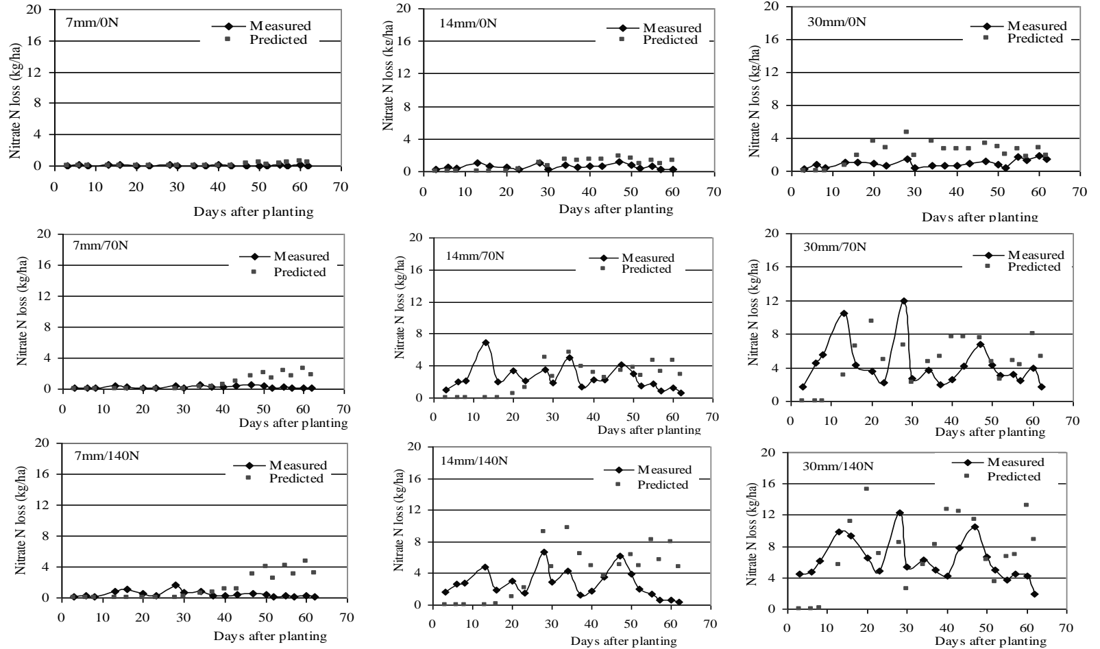
Figure 1. LEACHM-N simulated vs measured \text{NO}_3^- -N losses from the lysimeters at different treatment combinations in Yala 200F5.
